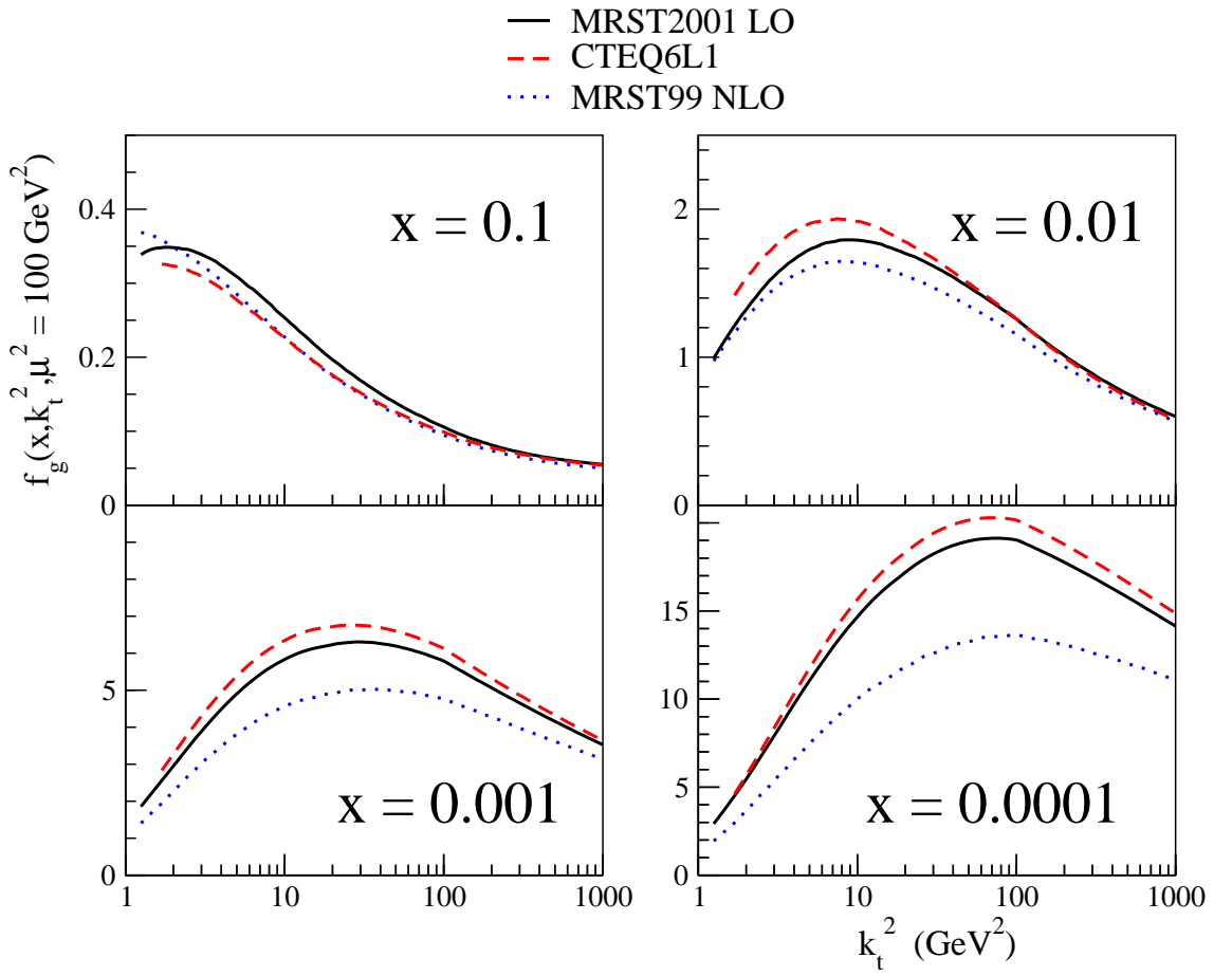
Figure 2.2: Sample plots of the unintegrated gluon distribution with MRST2001 LO, CTEQ6L1 and MRST99 NLO PDFs as input.
