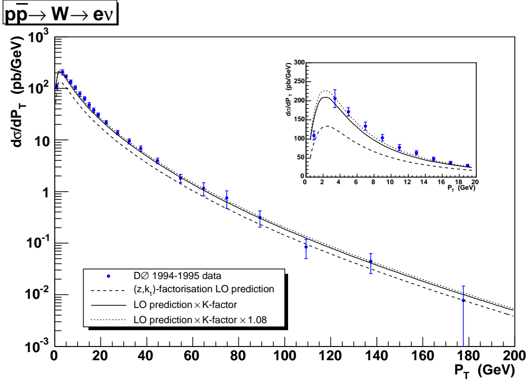
Figure 3.6: P_T distribution of W bosons compared to DØ data [105].
