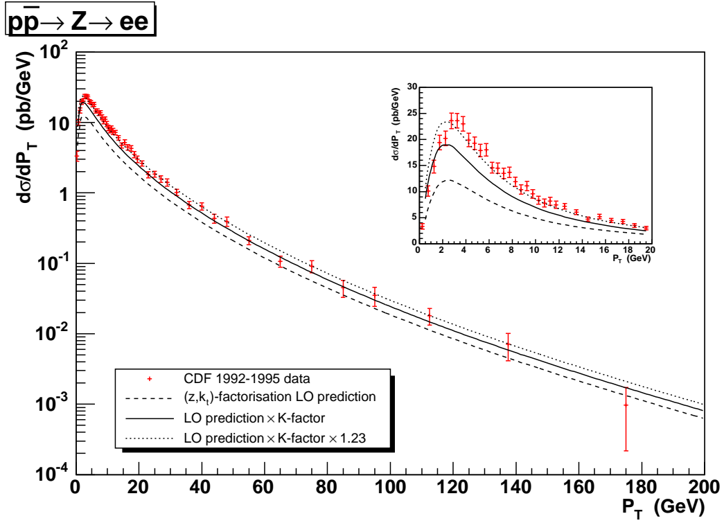
Figure 3.4: P_T distribution of Z bosons compared to CDF data [103].
