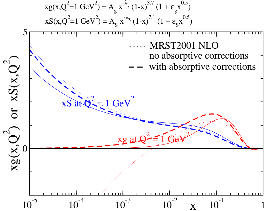
Figure 6.10: The input gluon and sea quark distributions obtained from a NLO DGLAP fit to F_2 , before and after absorptive corrections have been included, and taking a positive input gluon parameterisation. For reference the MRST2001 NLO input PDFs are also shown.
