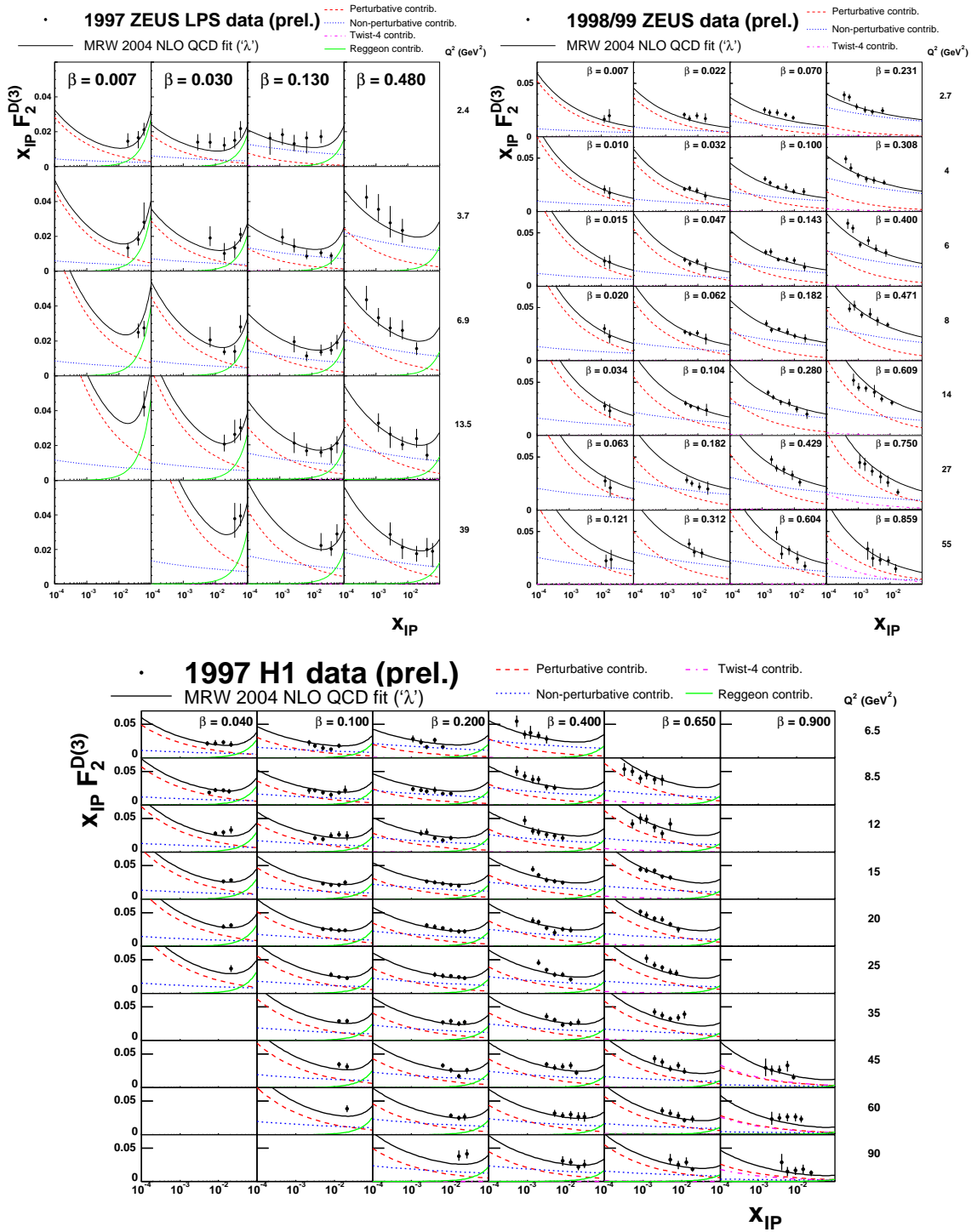
Figure 5.2: Fit to combined preliminary ZEUS [157, 158] and H1 [148] F_2^{D(3)} data with a ‘dummy’ gluon distribution of the proton proportional to x_{\bar{P}}^{-\lambda} (5.28). The curves show the four contributions to the total, as defined in (5.23). Only data points included in the fit are plotted.
