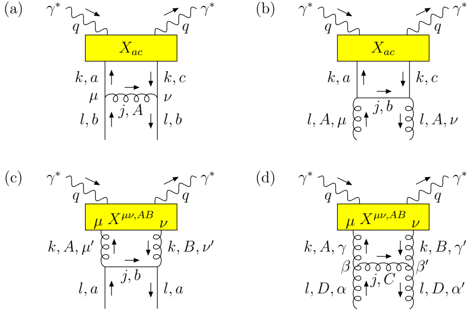
Figure 2.7: Cut diagrams giving the LO DGLAP splitting kernels: (a) P_{qq}(z) , (b) P_{gg}(z) , (c) P_{gq}(z) , (d) P_{qg}(z) . Here, j, k, l, q are momenta, a, b, c = 1, \dots, N_C and A, B, C, D = 1, \dots, (N_C^2 - 1) are colour indices, and \alpha, \beta, \gamma, \mu, \nu, \alpha', \beta', \gamma', \mu', \nu' are Lorentz indices. In each case, the box labelled X contains additional Lorentz and colour structure.
