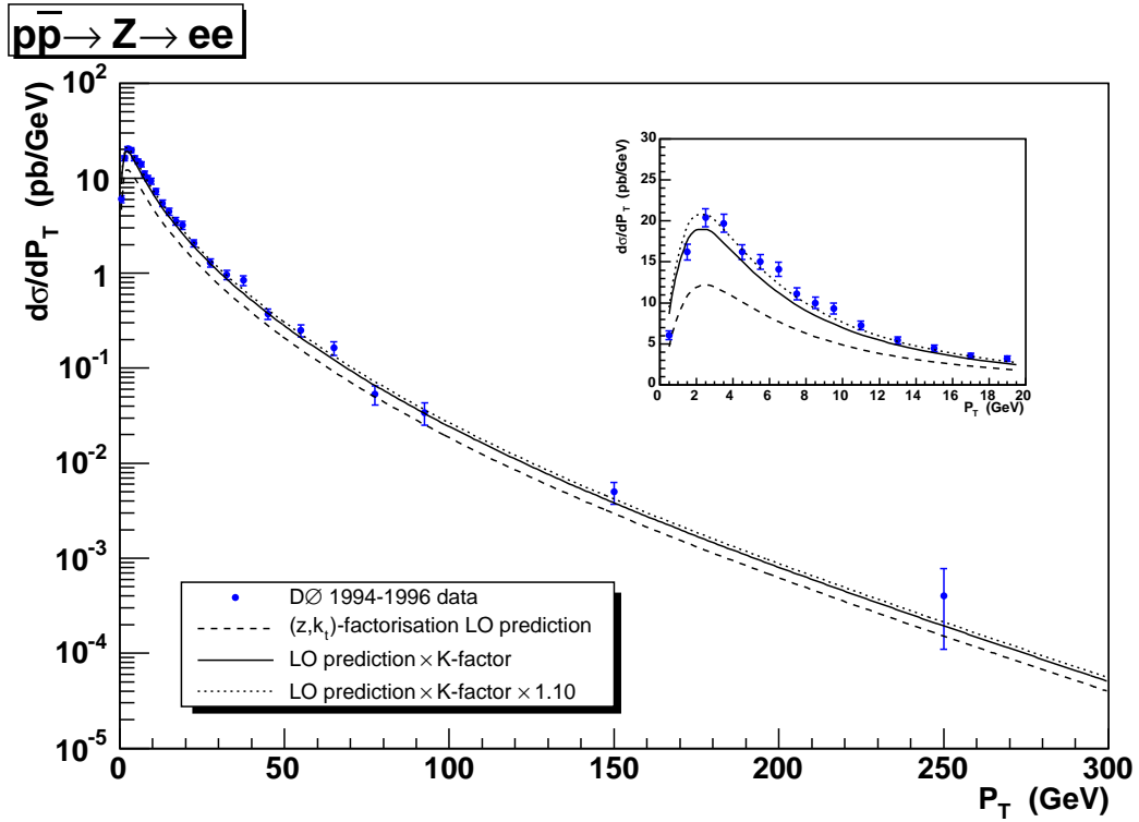
Figure 3.5: P_T distribution of Z bosons compared to DØ data [104].
