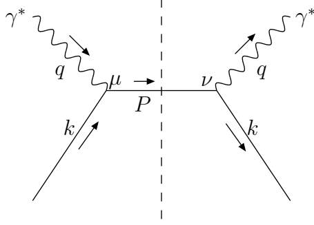
Figure 2.9: Cut diagram contributing at LO in the (z, k_t) -factorisation approach.
