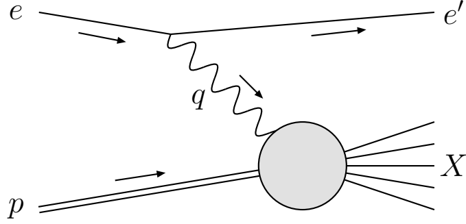
Figure 1.1: Deep-inelastic ep scattering mediated by a virtual photon \gamma^* .
