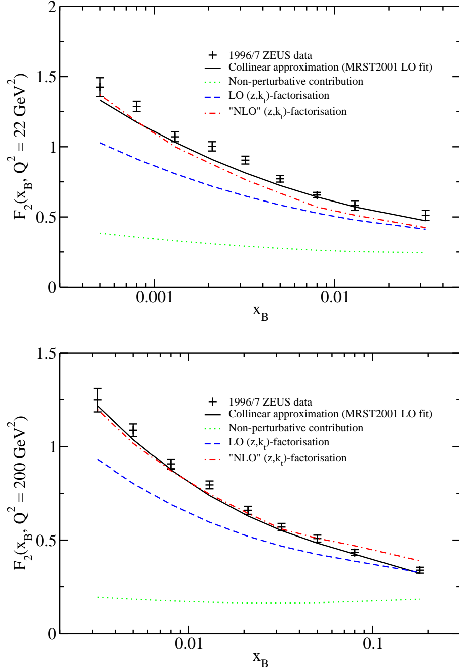
Figure 3.9: Predictions for F_2(x_B, Q^2) at Q^2 values of 22 \text{GeV}^2 (top) and 200 \text{GeV}^2 (bottom) in the collinear approximation, where the 1996/97 ZEUS data [111] has been included in the MRST2001 LO fit [66], and in the (z, k_t) -factorisation approach using the same PDFs as input. The discrepancy between the data and the LO (z, k_t) -factorisation prediction can be eliminated by either refitting the input integrated PDFs or by adding some 'NLO' contribution.
