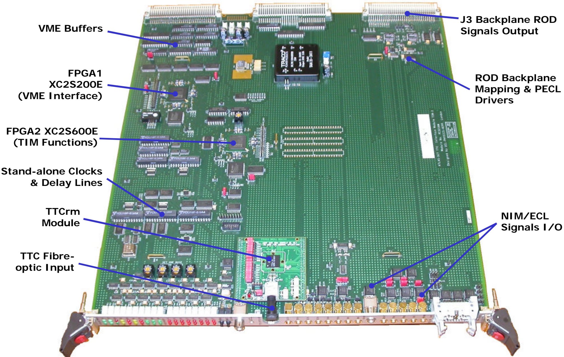
TIM-3A Functional Layout
