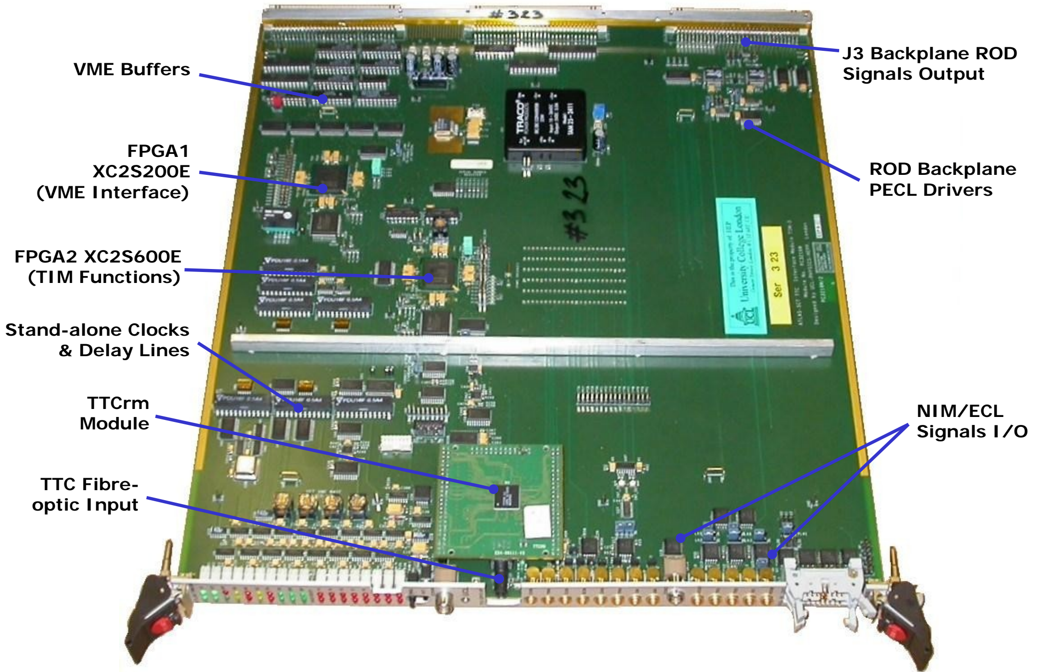
TIM-3B Functional Layout
