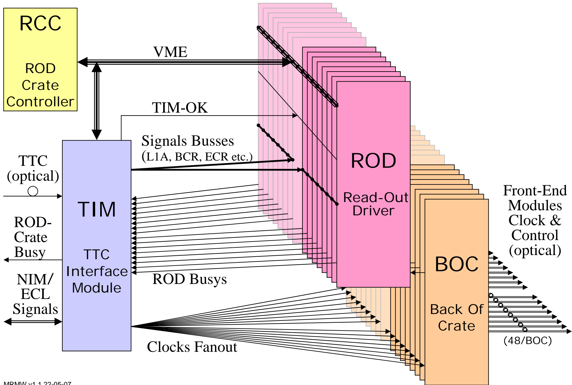
TIM Connections Overview
