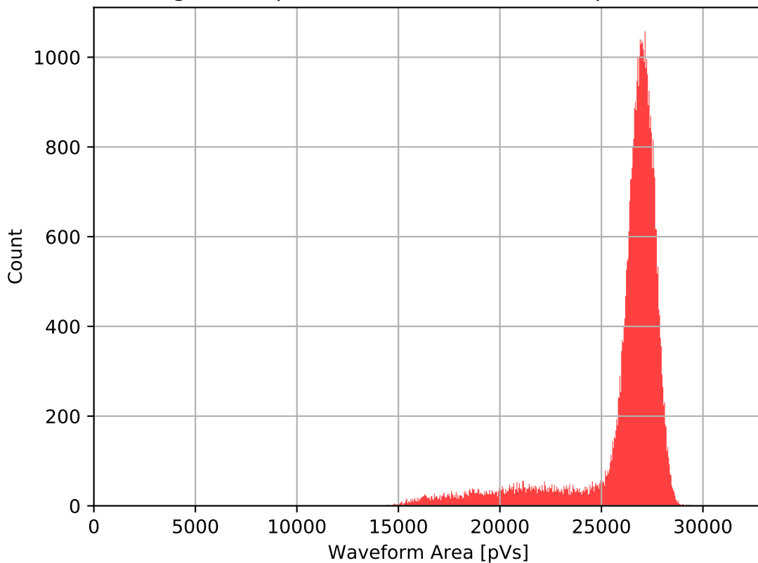
Histogram output from HDO6104 Oscilloscope - 500 bins
