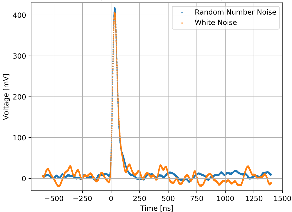
Example Emulated Signals with Noise Output from HDO6104 Oscilloscope
