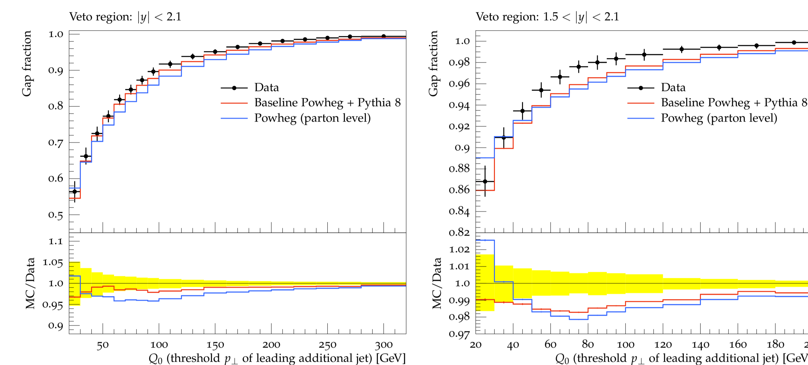
Figure 2: Gap fractions in the inclusive and the problematic veto region. Comparison of baseline MC prediction and prediction of Powheg NLO matrix elements alone to ATLAS data. Error bars show statistical uncertainty, yellow band shows statistical and systematic uncertainty added in quadrature.
