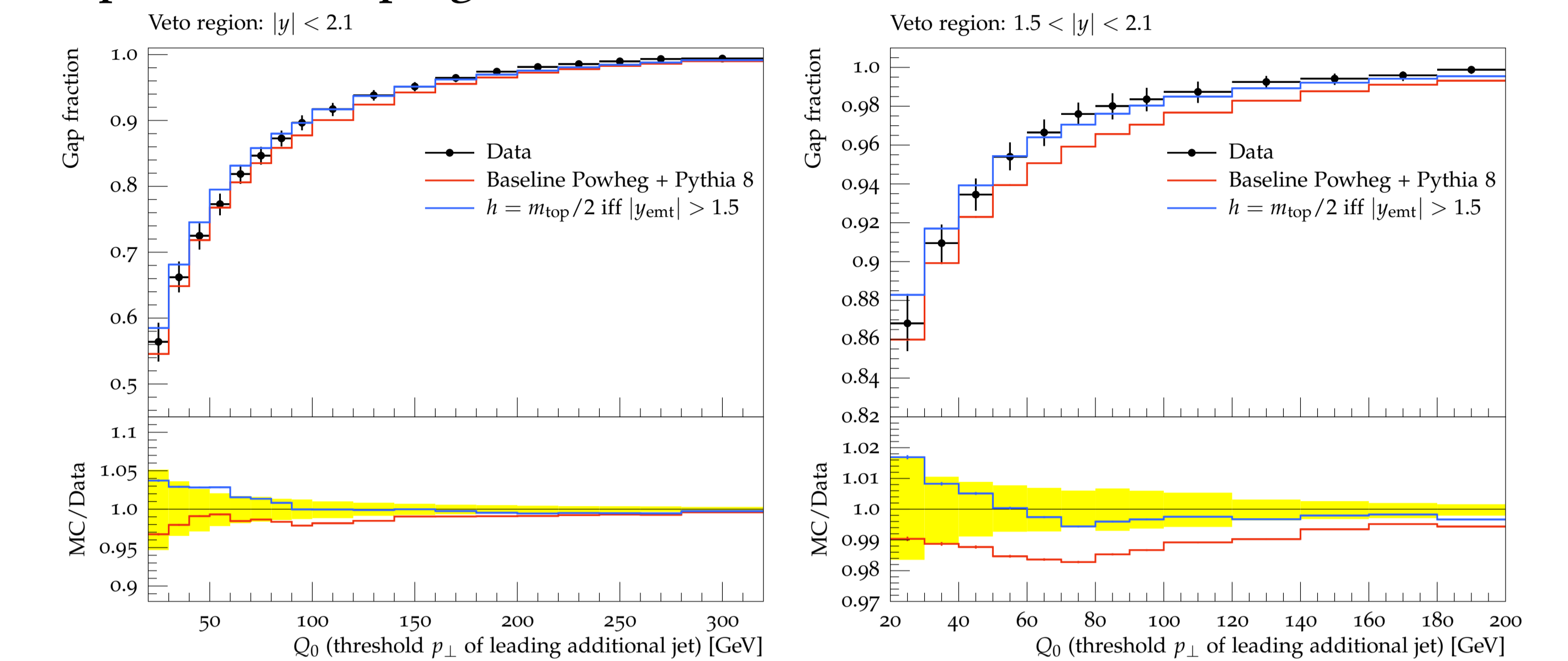
Figure 3: Damping resummation for emissions with |y| > 1.5 in Powheg. Agreement in the problematic rapidity region (right) has been achieved!
