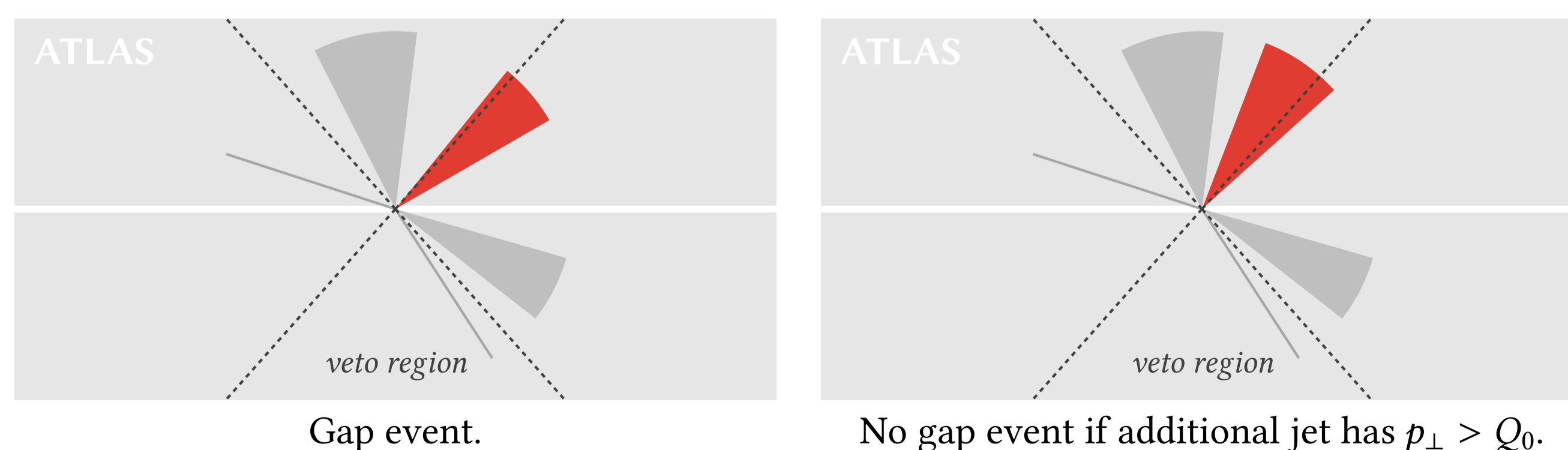
Figure 1: Simple examples of t\bar{t} events with and without gap. Shown in red is the leading additional jet and in gray the two b-jets and leptons from t\bar{t} decay. The veto region is indicated by dashed lines, assuming massless additional jets, so that y = \eta .
