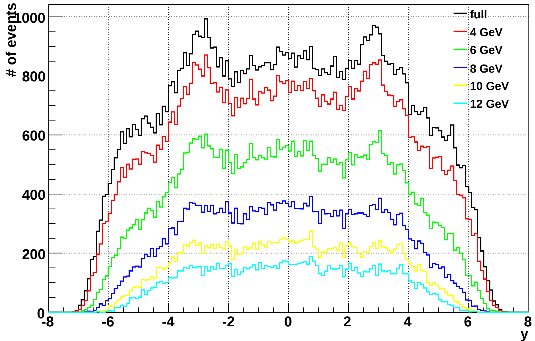
drell-yan pair rapidity distribution
