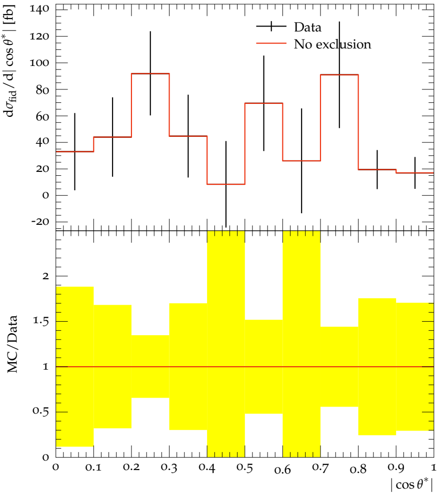
Photon decay angle in the Collins-Soper frame
