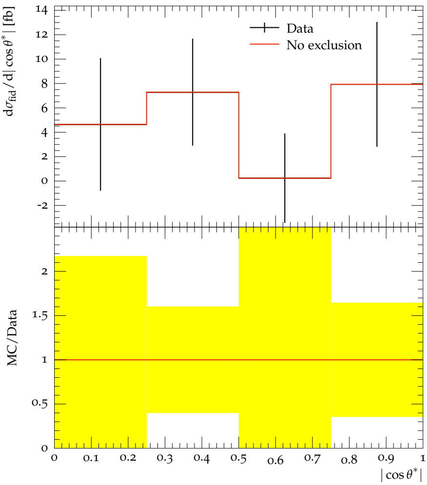
Photon decay angle in the Collins-Soper frame, 80 < p_T^{\gamma\gamma} < 200 Ge
