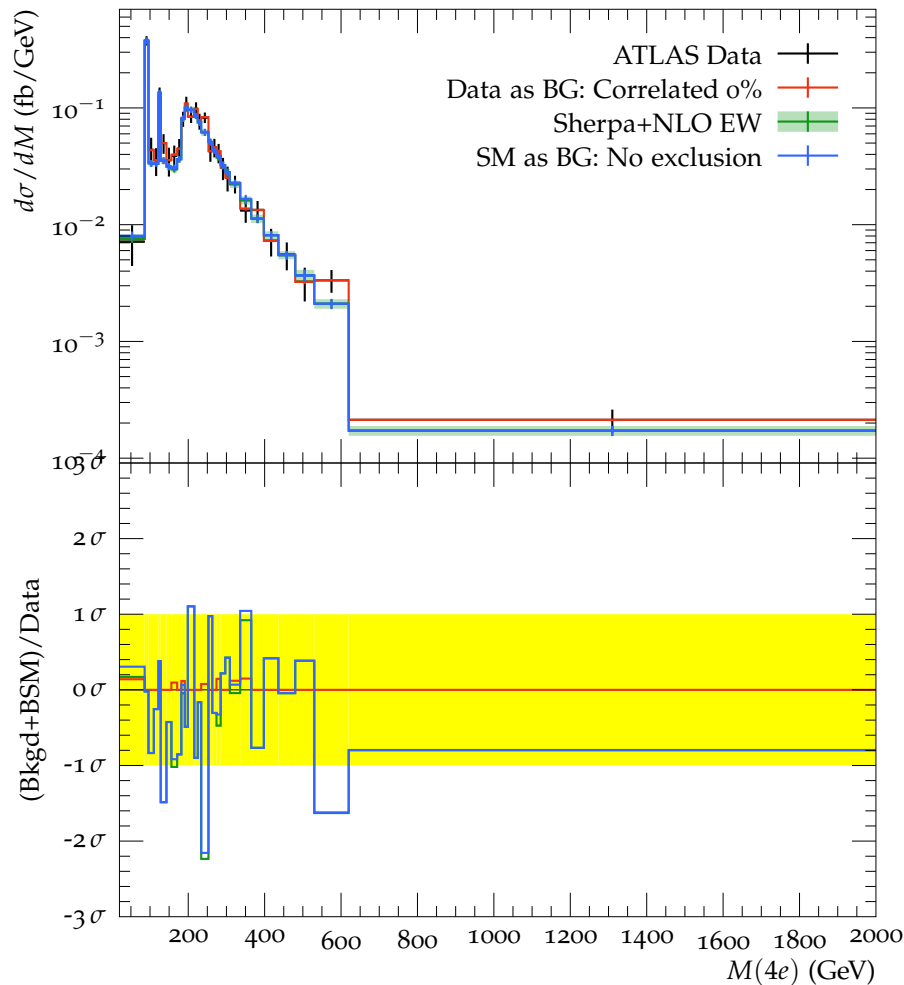
Inclusive differential cross section for four electrons (Max = 887 GeV)
