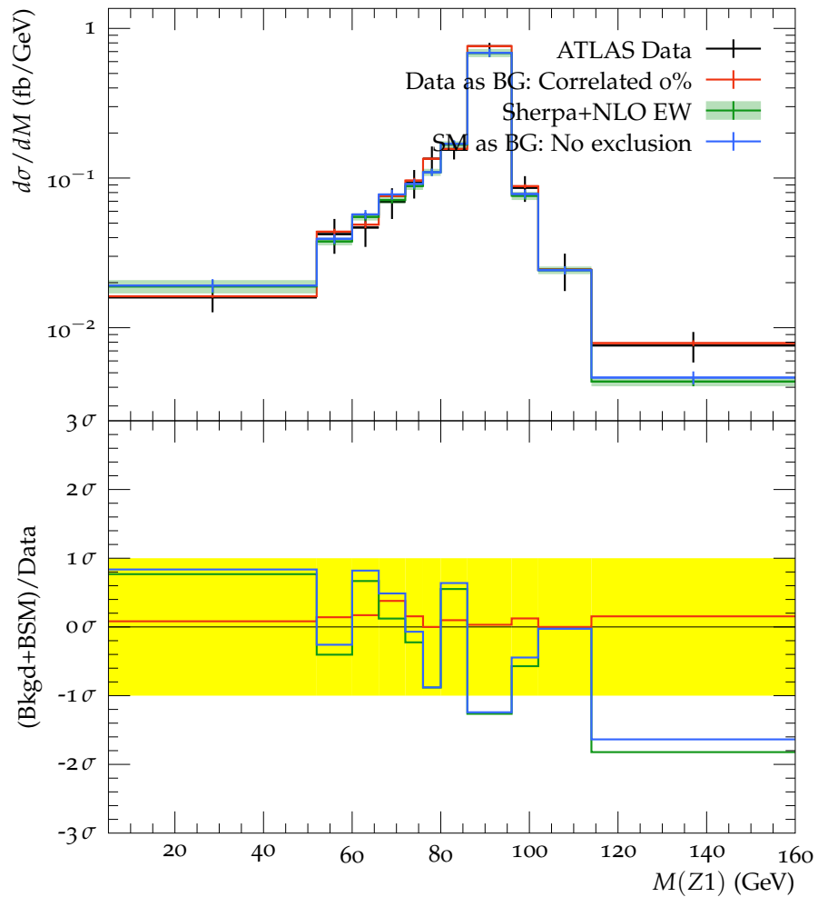
Mass of the first dilepton pair in the offshell region (Max = 146 Ge)
