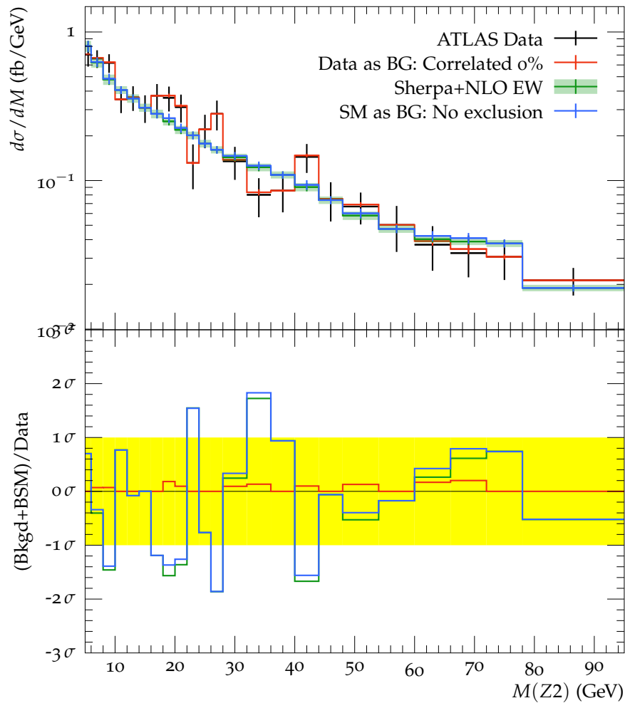
Mass of the second dilepton pair in the offshell region (Max = 88.3
