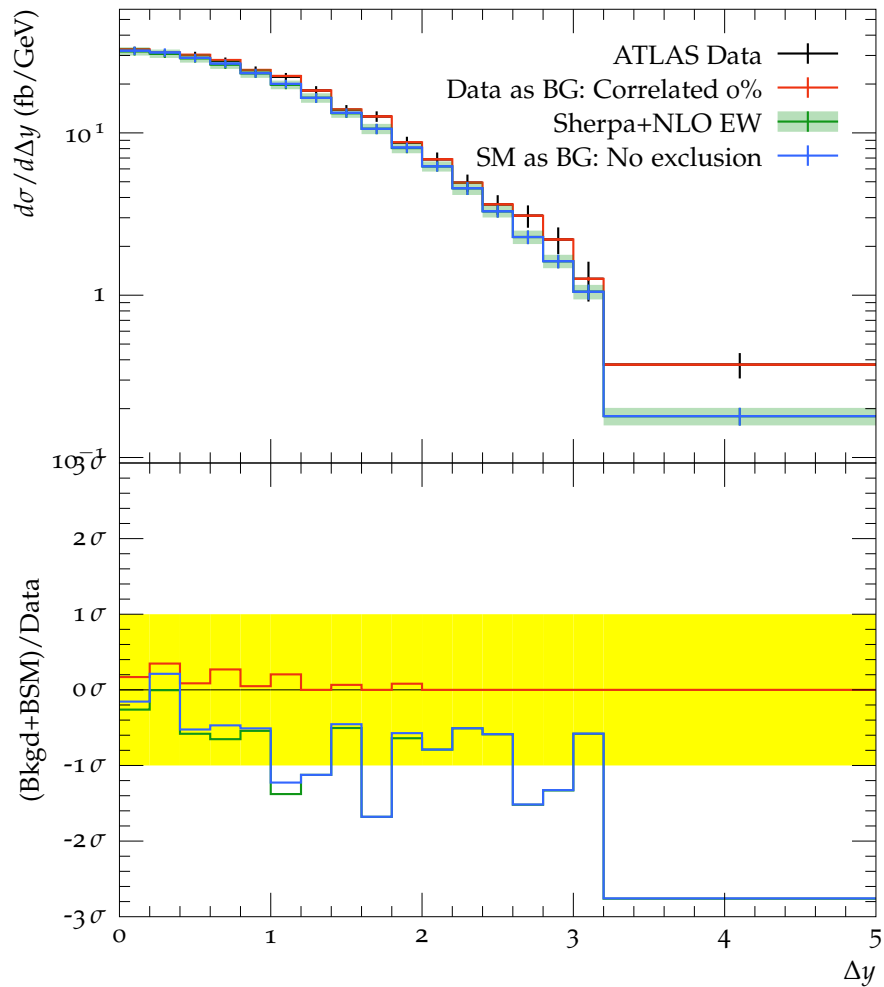
\Delta y between the dilepton pairs in the ZZ mass region.
