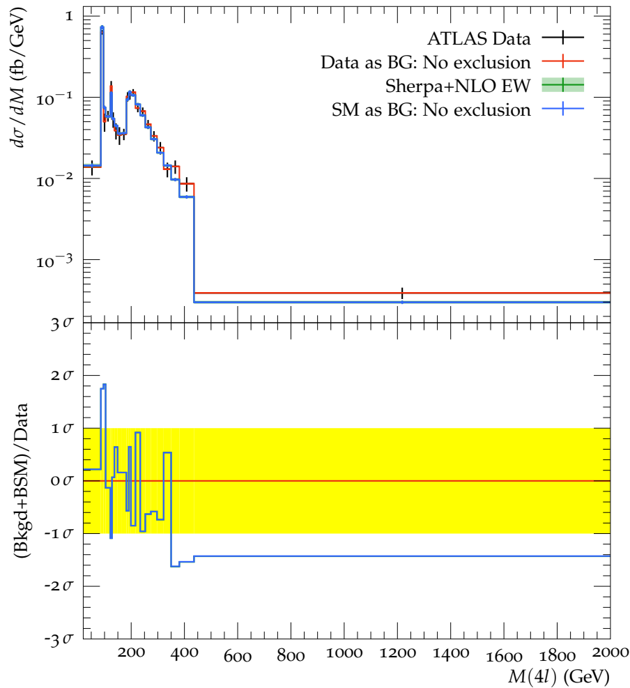
Four lepton mass in first p_T^{4l} slice (Max = 726 GeV)
