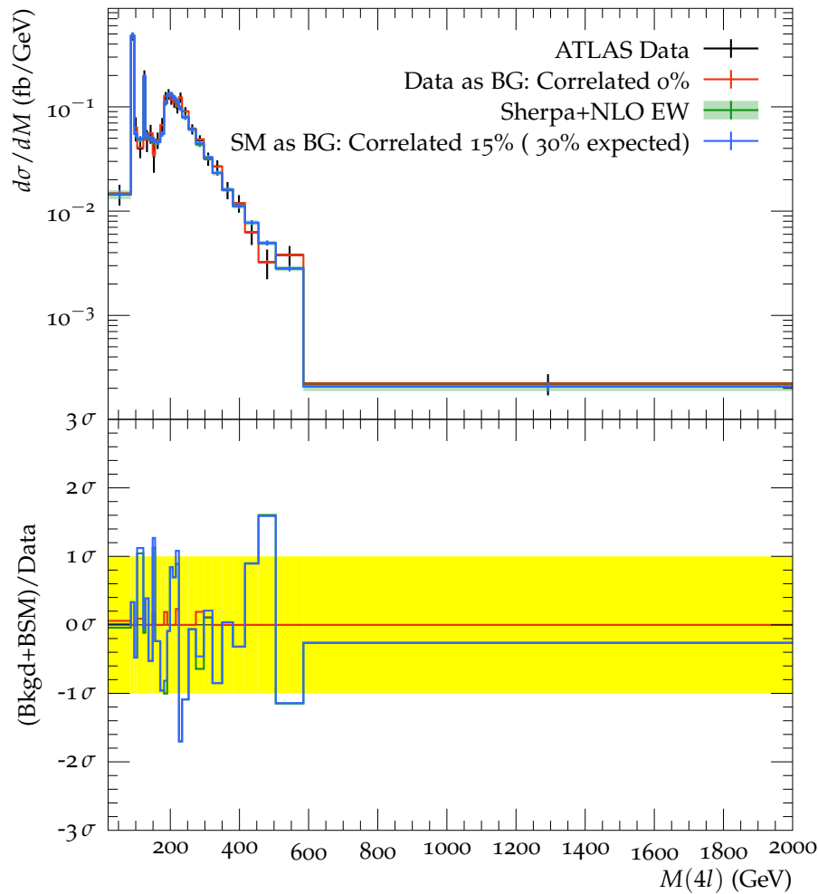
Four lepton mass in third p_T^{4l} slice (Max = 1153 GeV)
