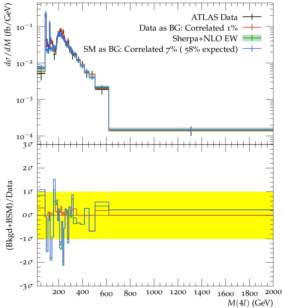
Four lepton mass in fourth p_T^{4l} slice (Max = 1320 GeV)
