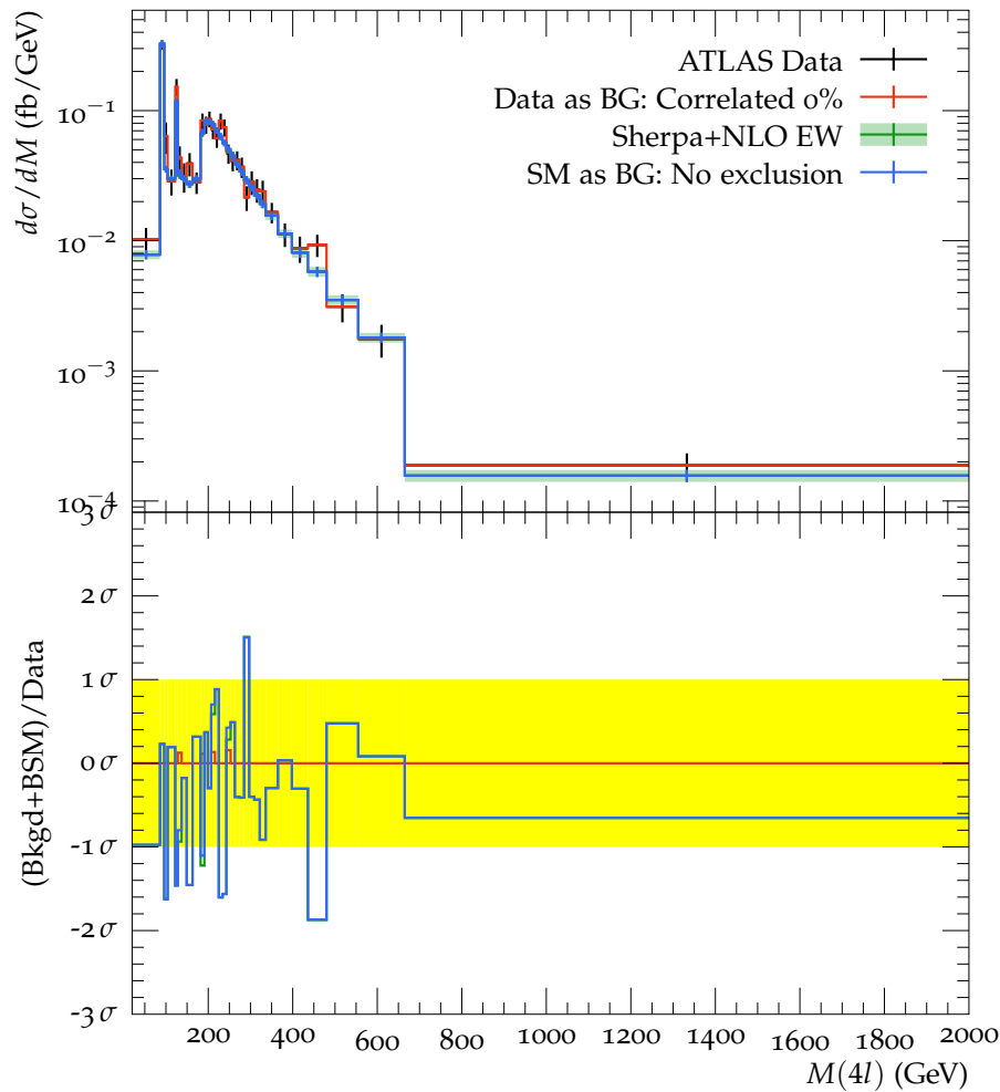
Four lepton mass in second y^{4l} slice (Max = 1116 GeV)
