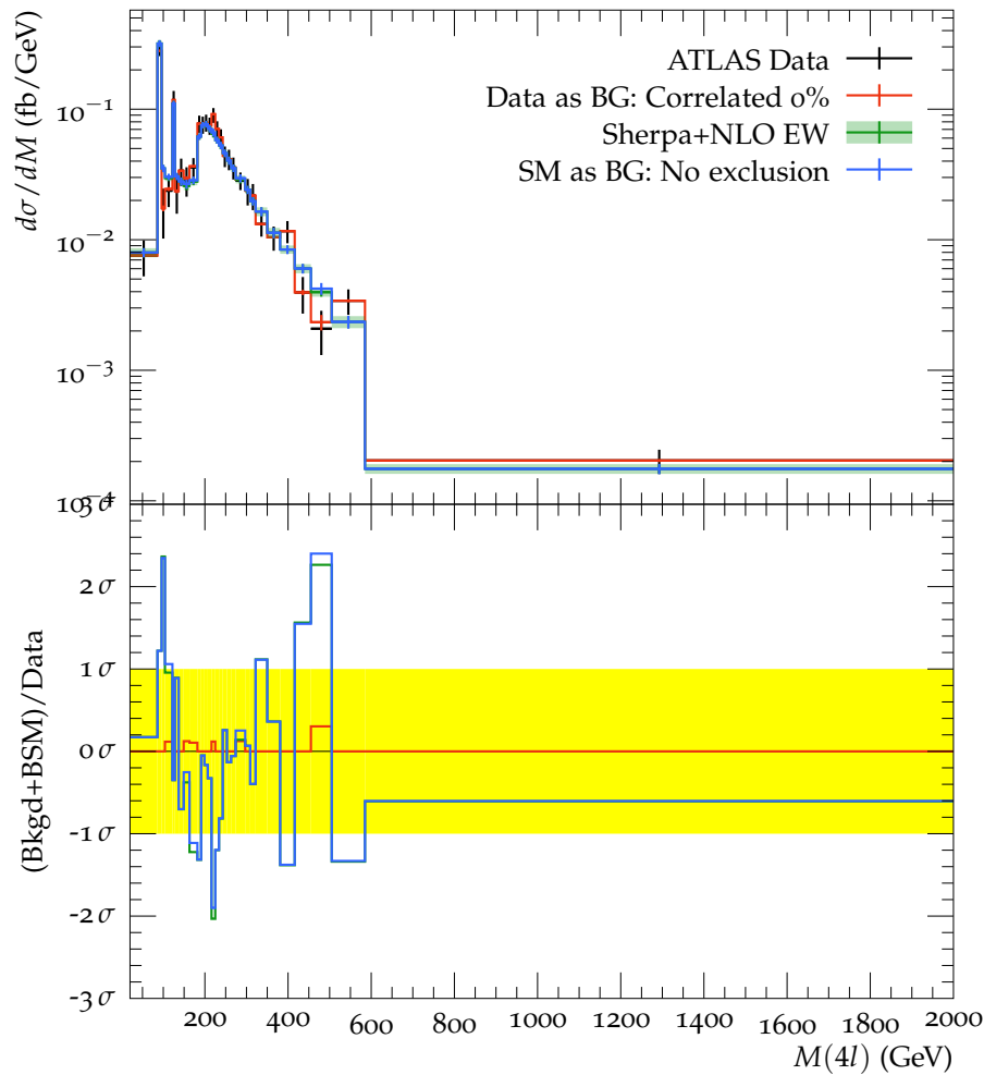
Four lepton mass in third y^{4l} slice (Max = 1413 GeV)
