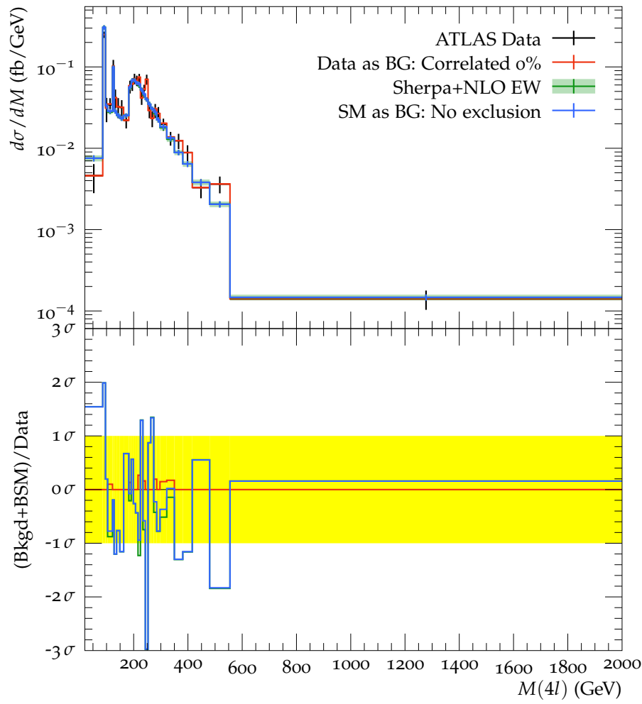
Four lepton mass in fourth y^{4l} slice (Max = 1044 GeV)
