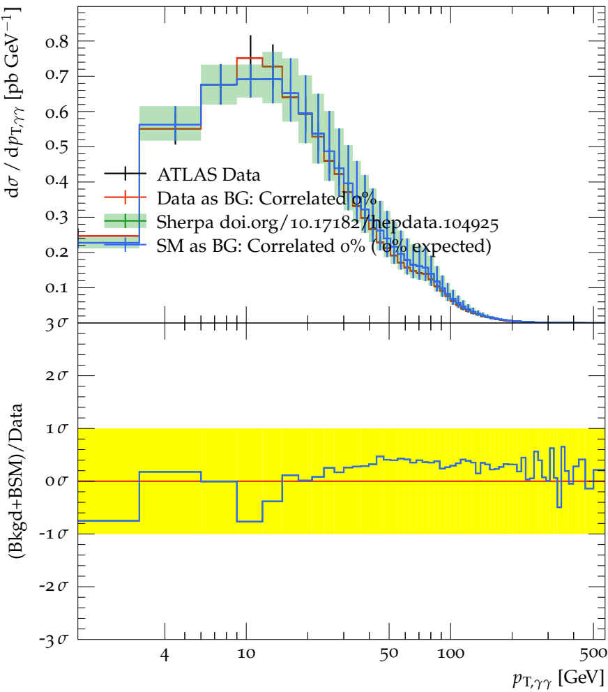
p_T of the diphoton system
