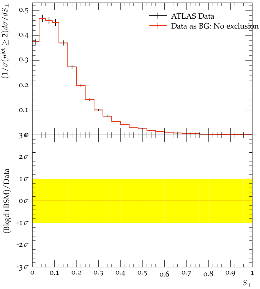
Transverse Sphericity for n^{\text{jet}} = 4 , H_{T2} > 2.0 TeV
