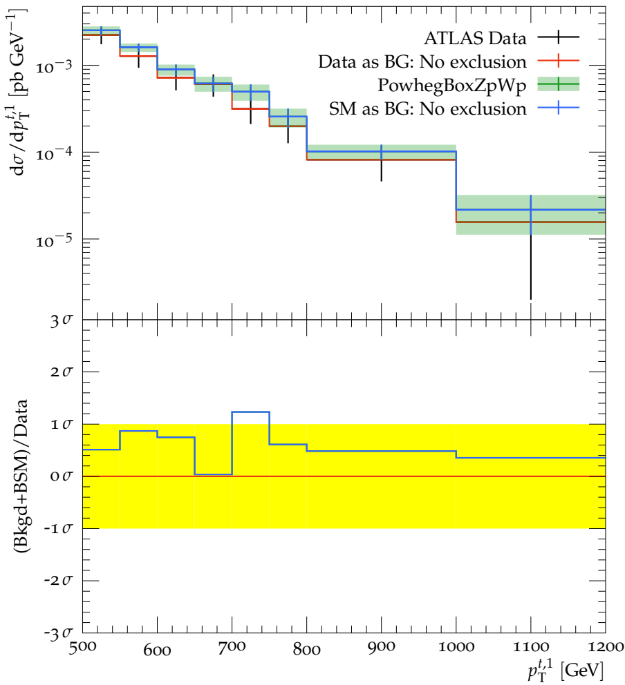
Particle-level leading top transverse momentum
