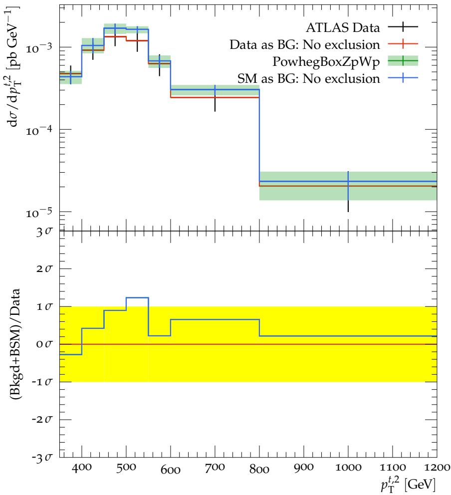
Particle-level subleading top transverse momentum
