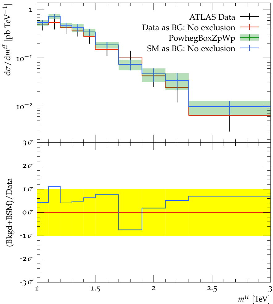
Particle-level t\bar{t} invariant mass
