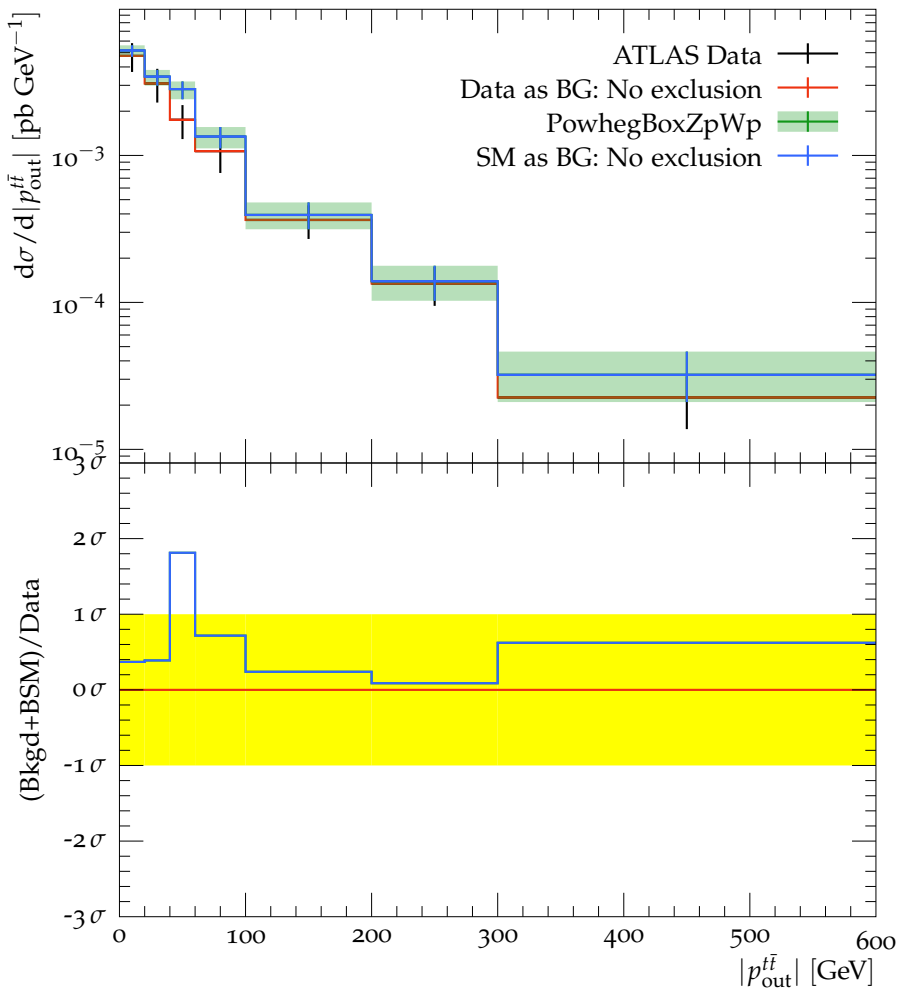
Particle-level t\bar{t} out-of-plane momentum
