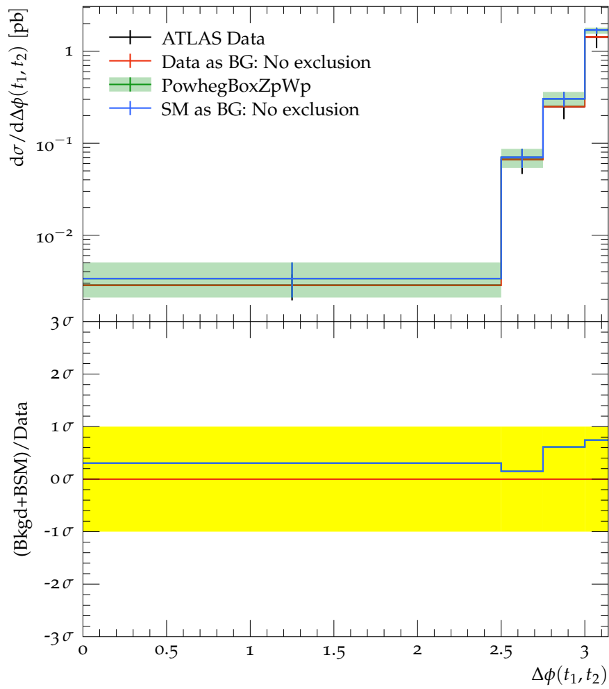
Particle-level t\bar{t} azimuthal opening angle
