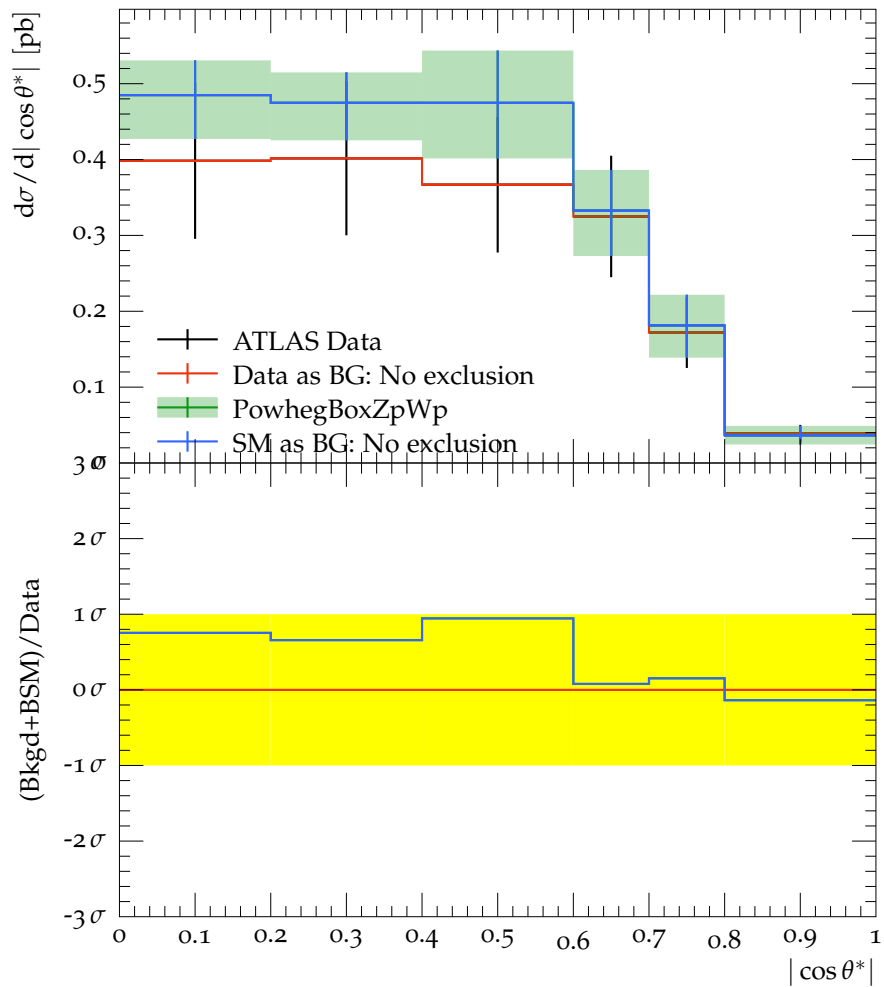
Particle-level t\bar{t} \cos \theta^*
