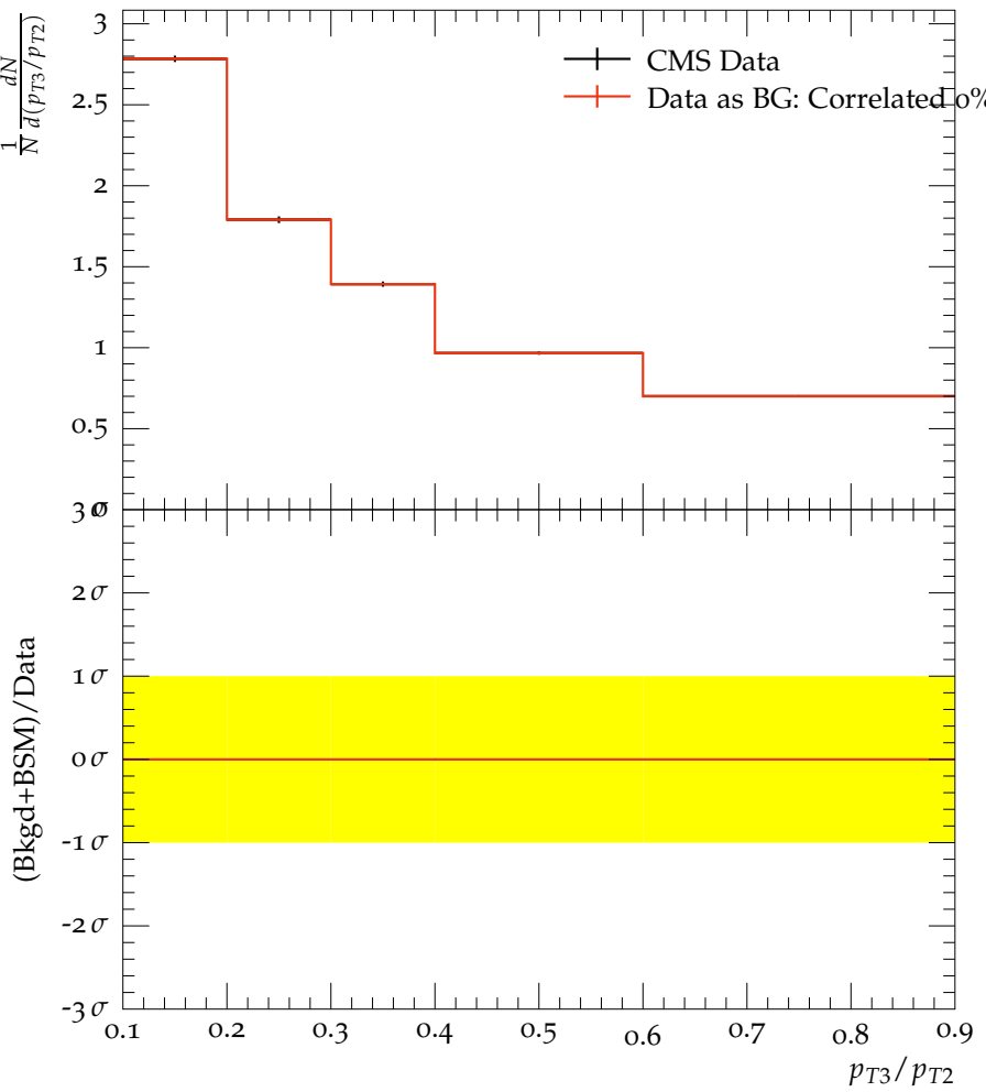
CMS, 13 TeV, Three-jet p_{T3}/p_{T2} for small-angle radiation
