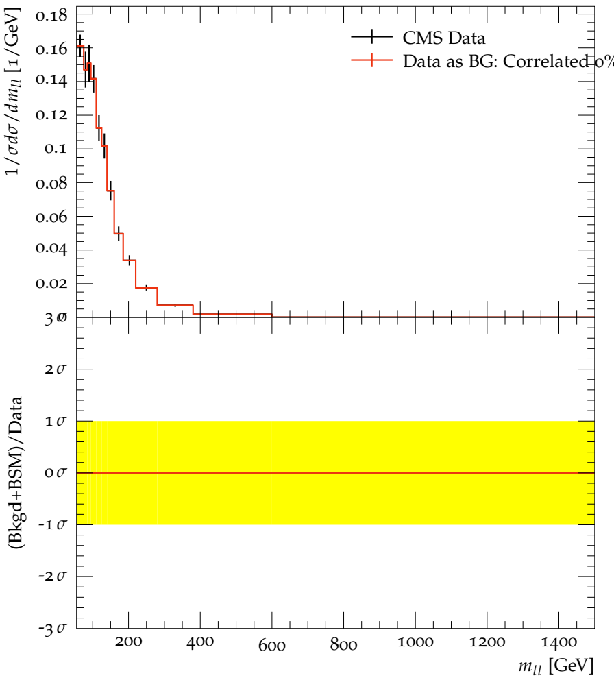
CMS, 13 TeV, W^+W^- , Figure 6 upper left
