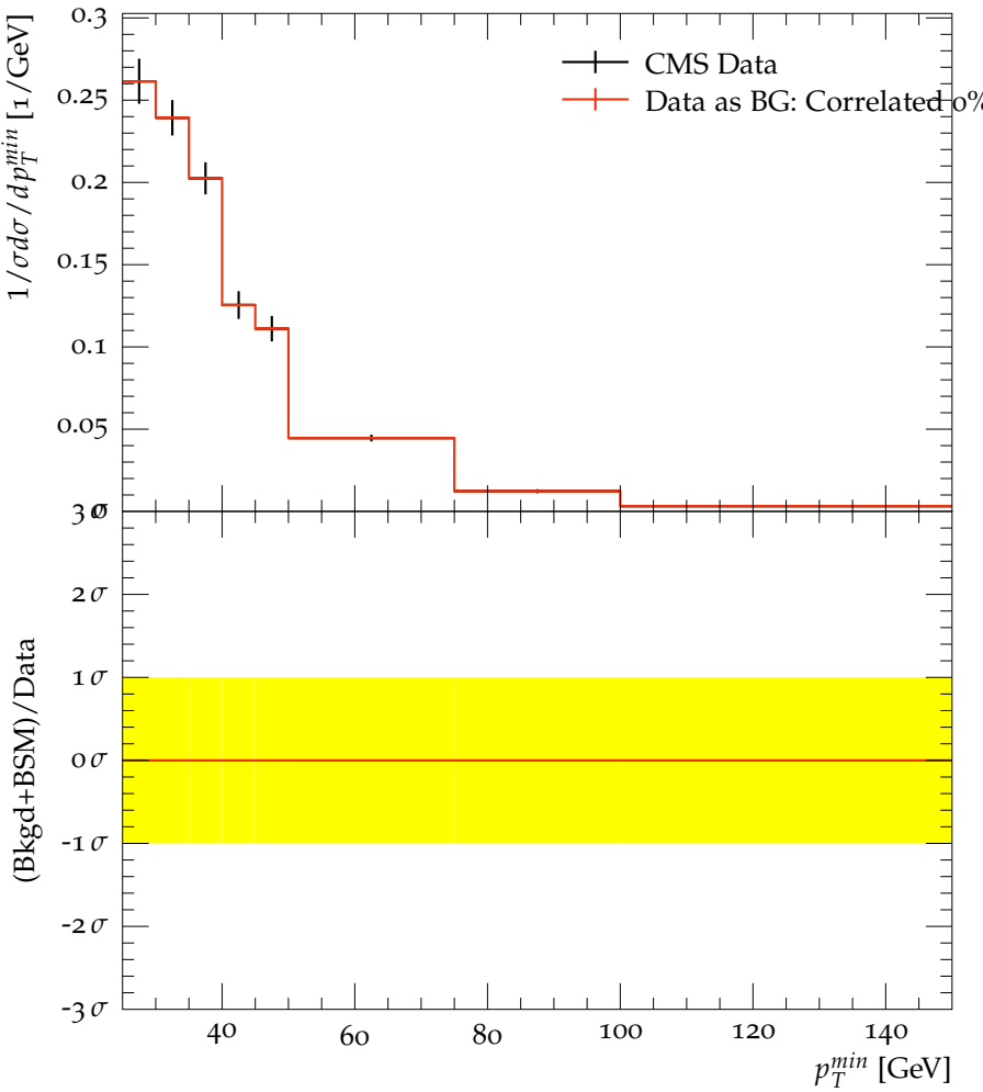
CMS, 13 TeV, W^+W^- , Figure 6 lower left
