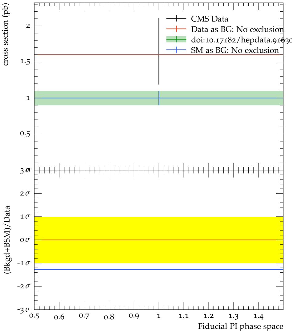
CMS, 13 TeV, t\bar{t}b\bar{b} all-jets fiducial PI cross section
