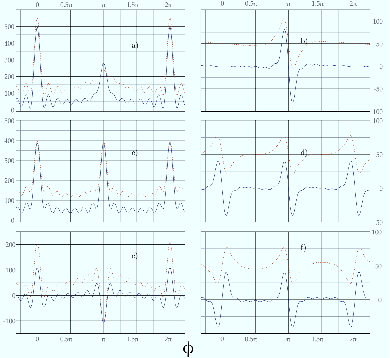
Figure 6: The reverse Fourier transform using the average coefficients over the colour singlet sample without underlying event (blue solid curve) and the QCD di-jets with underlying event (red dashed curve). a) uses only the real part of the coefficients, b) only the imaginary part. c) uses only the real even coefficients, d) uses only the imaginary even coefficients. e) uses the real odd coefficients and f) uses the imaginary odd coefficients. For all but a) and c) the red dashed curve has been raised by 50 GeV in order to separate it from the blue solid curve.
