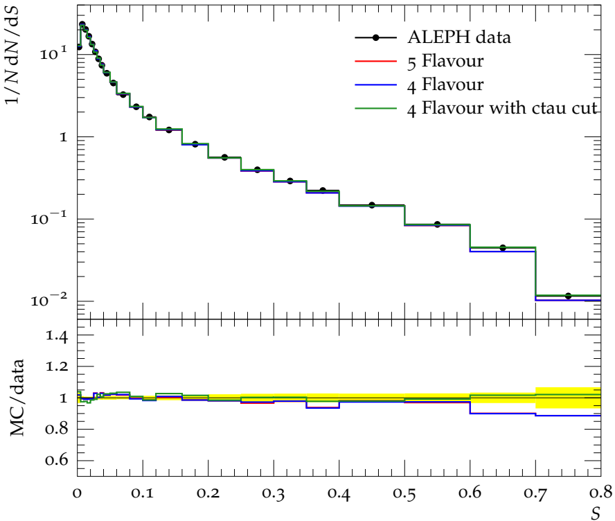
Sphericity, S (charged)
