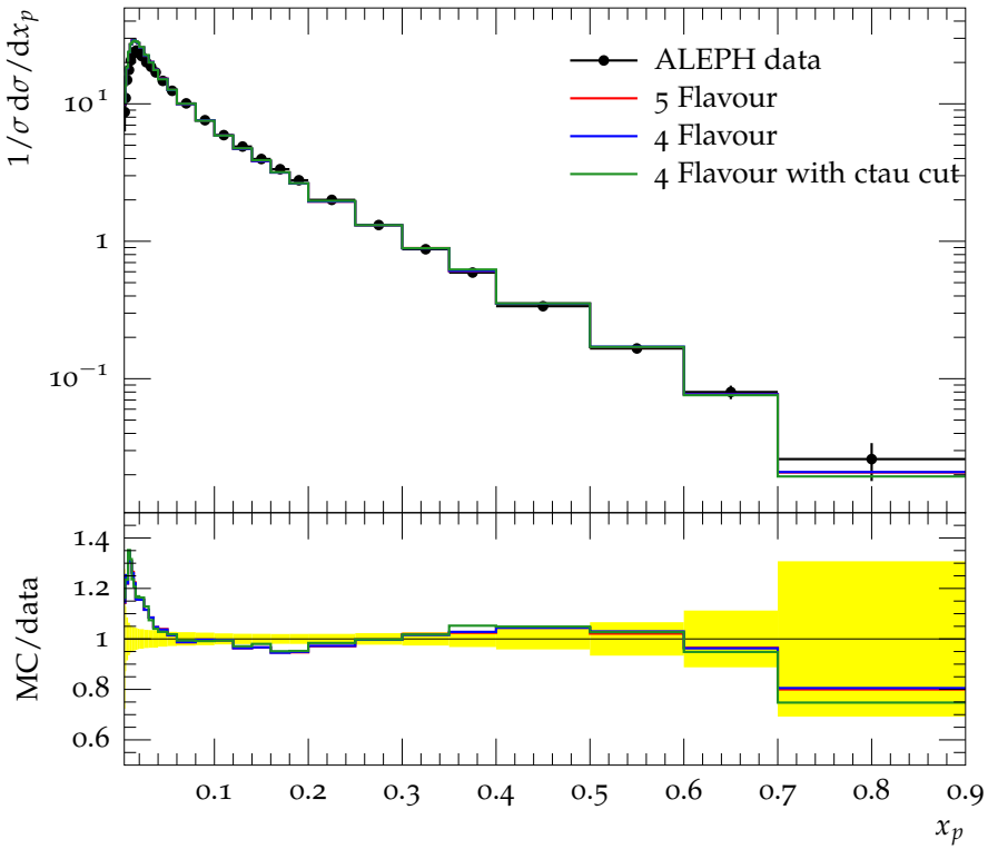
K^0 spectrum
