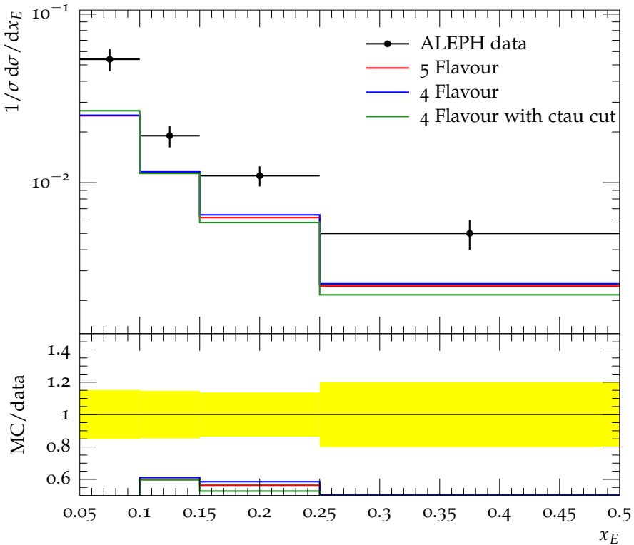
\Xi^0(1530) spectrum
