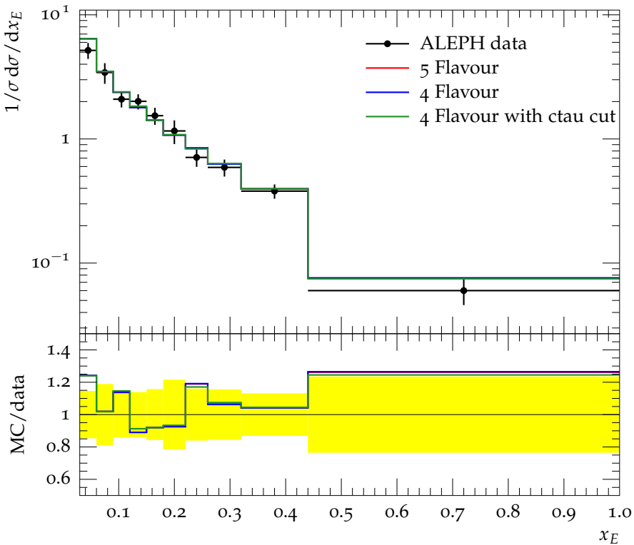
K^{*\pm}(892) spectrum
