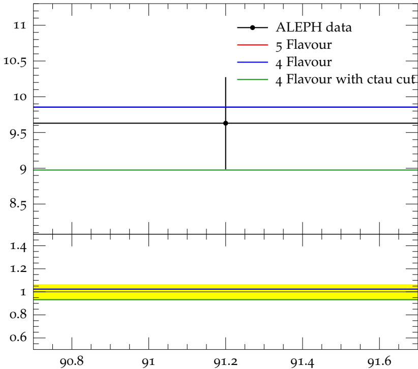
Mean \pi^0 multiplicity
