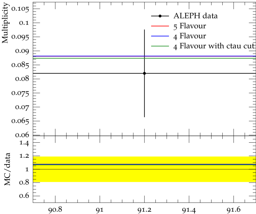
Mean \Sigma multiplicity
