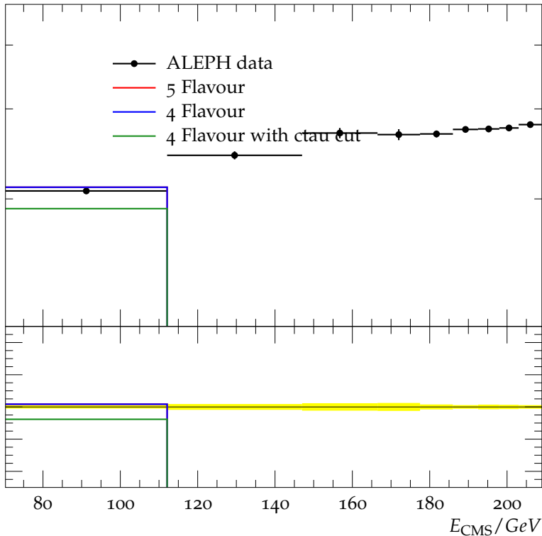
Charged multiplicity at a function of energy
