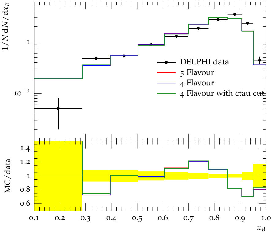
b quark fragmentation function f(x_B^{\text{prim}})
