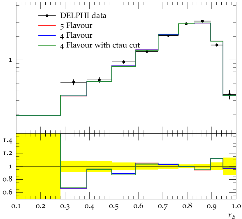
b quark fragmentation function f(x_B^{\text{weak}})
