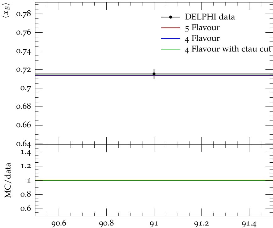
Mean of b quark fragmentation function f(x_B^{\text{weak}})
