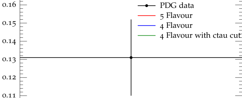
Mean D^+s multiplicity
