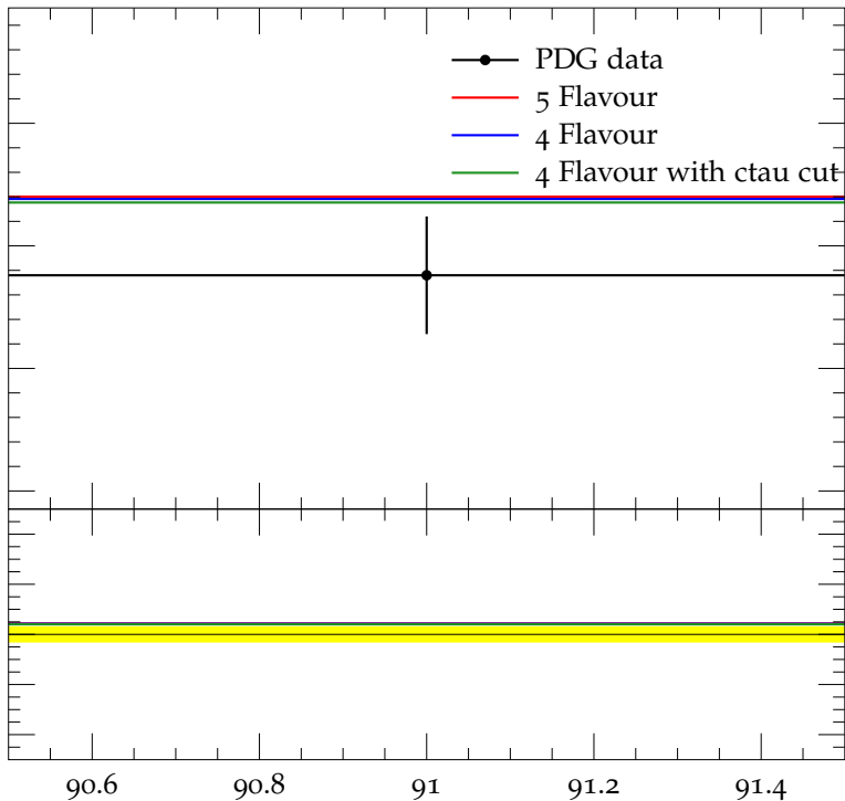
Mean K^{*0}(892) multiplicity
