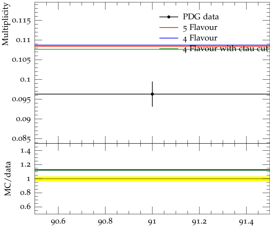
Mean \phi(1020) multiplicity
