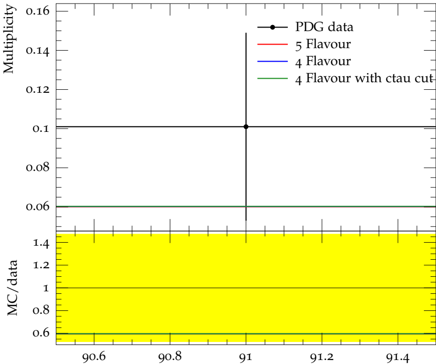
Mean D_s^{*+}(2112) multiplicity
