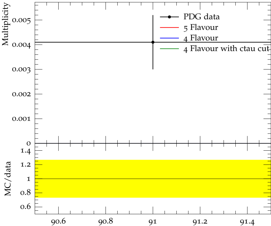
Mean \chi_{c1}(3510) multiplicity
