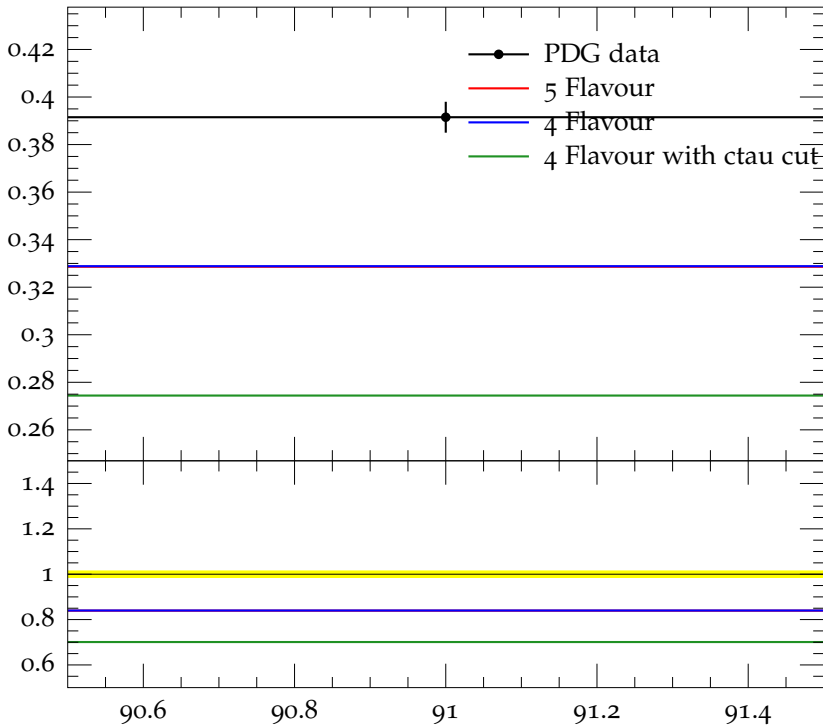
Mean \Lambda multiplicity
