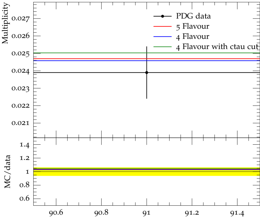
Mean \Sigma^+(1385) multiplicity
